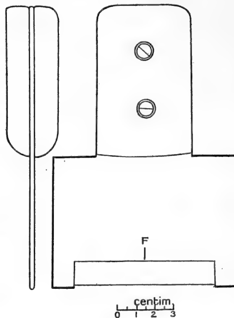
TEXT-FIG. 48. Knife for decerebrator, showing the rounded end-shoulders protecting the cutting edge.
